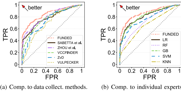
Fig. 14. ROC curves for true positive rate (TPR) and false positive rate (FPR). We compare FUNDED to other automatic data collection frameworks (a) and individual expert models used in our expert committee (b). Methods that give curves closer to the top-left corner indicate a better performance.
