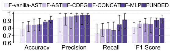
Fig. 17. Comparing implementation variants of FUNDED. Our implementation gives the best overall performance.
