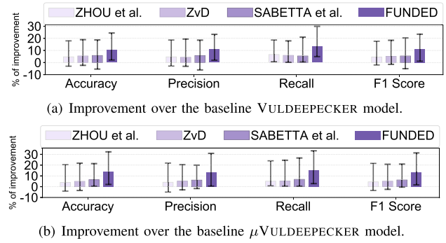
Fig. 15. Performance improvement over the baseline code detection models when using extra labeled training samples from GitHub. The min-max bar shows the range of improvement across the top-10 CWE vulnerability types.
