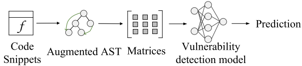
Fig. 3. Code vulnerability detection. Our detection model takes as input an AST and CDFG of the target code snippet at the function level.
