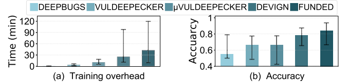
Fig. 19. Training overhead (a) and accuracy (b). The min-max bars show the variances across evaluation settings.
