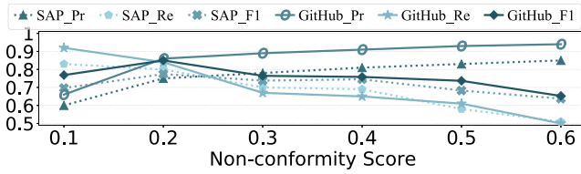
Fig. 20. How performance of our data labeling model changes as the non-conformity threshold increases on the SAP and Github datasets.
