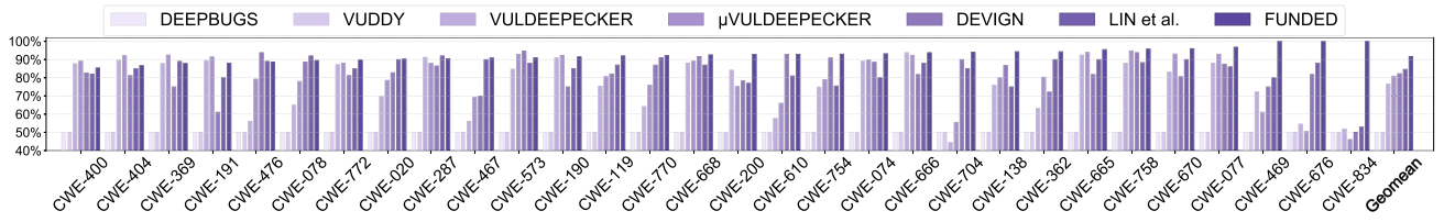
Fig. 16. Detection accuracy for the top-30 CWE vulnerability types on standard vulnerability databases.
