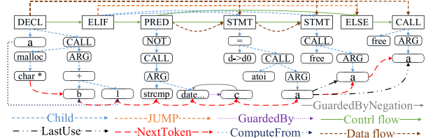
(b) Augmented AST
